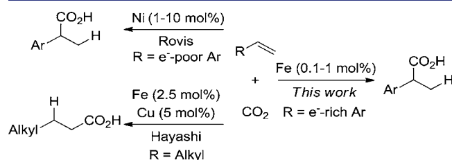
Figure 1. Proposed iron-catalyzed hydrocarboxylation of alkenes.
