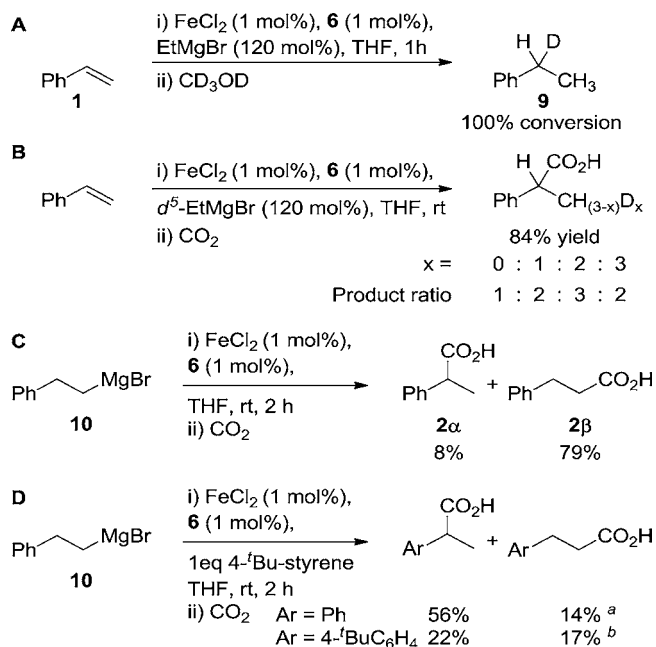
Scheme 1. Mechanistic Investigations into the Iron-Catalyzed Hydrometallation of Alkenes and Isomerization of Grignard Reagents a,b
